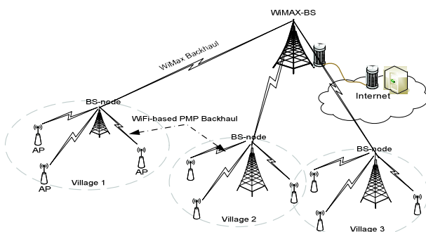
Figure 1. Wireless broadband network architecture.
