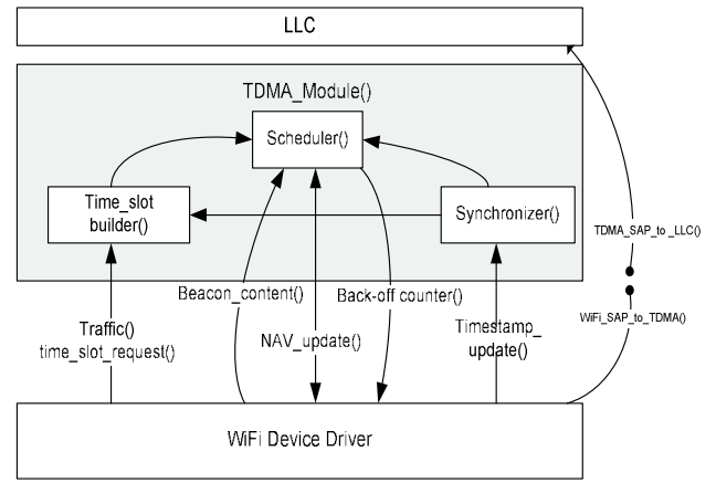
Figure 6. Cross-layer design for TDMA-based MAC.
