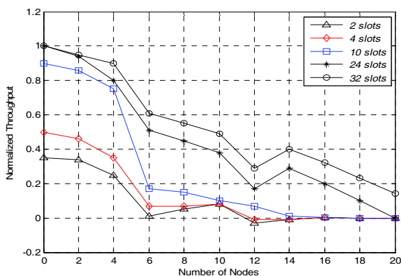
Figure 8. The normalized throughput vs number of nodes for different number of slot.
