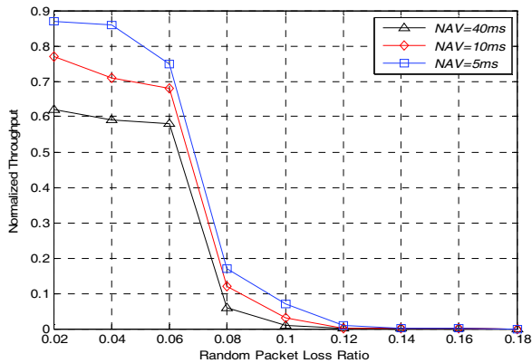
Figure 7. Normalized throughput and the random packet loss rate for different access time for the NAV update.
