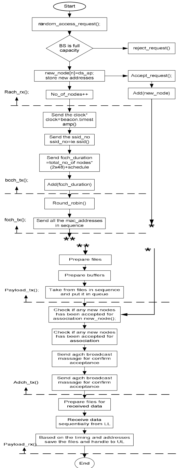
Figure 4. Flowchart for the TDMA-MAC protocol.
