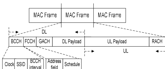
Figure 3. Additional TDMA header is added to WiFi frame.
