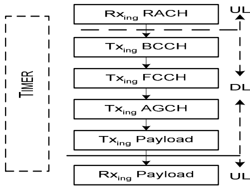
Figure 5. The flow of the virtual channels for the TDMA frame.
