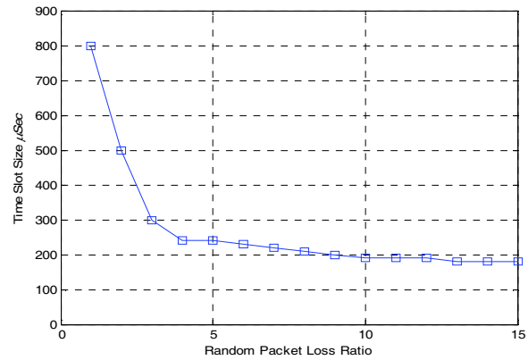
Figure 9. Time slots size vs. the packet loss ratio.
