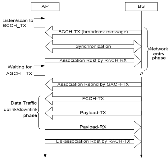
Figure 2. Protocol flow of the TDMA-based PMP.
