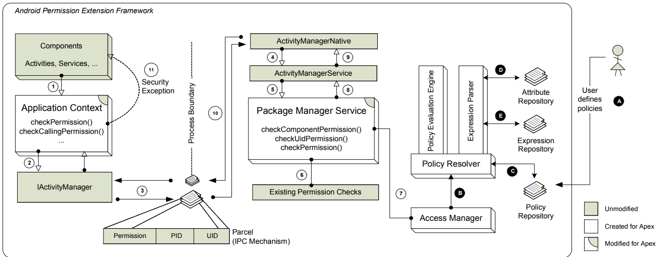
Figure 1. Apex architecture.
