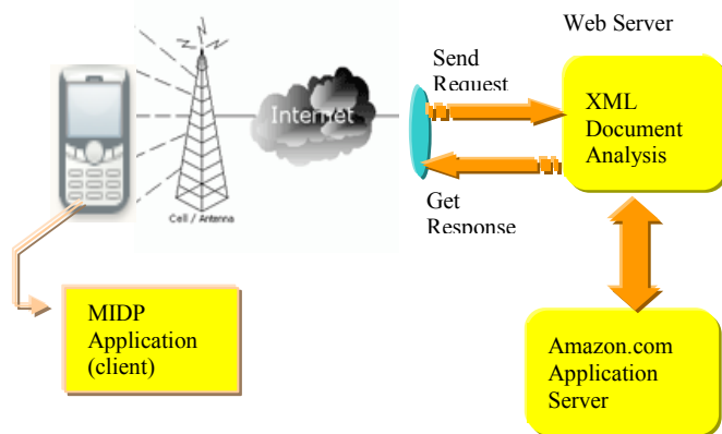
Figure 2. A detailed description of eCoMobile information retrieval process.
