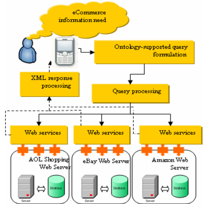
Figure 1. An abstract description of eCoMobile information retrieval process.
