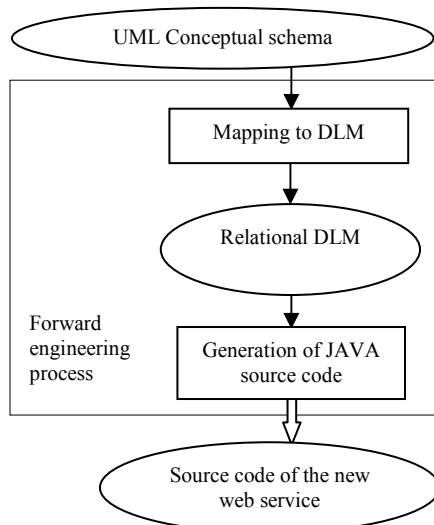
Figure 6. Forward engineering process.
