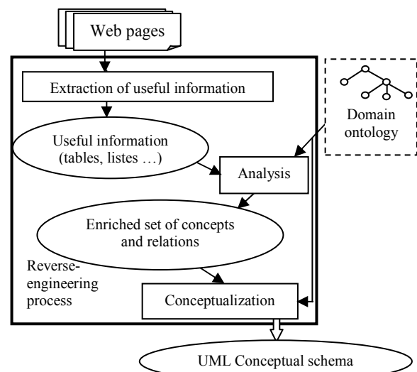
Figure 3. Ontology based web application reverse-engineering process.
