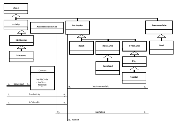
Figure 5. UML Conceptual schema of the chosen site.
