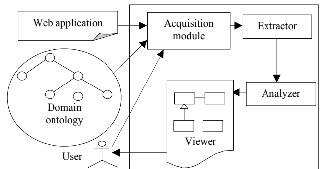
Figure 4. OntoWeR architecture.
