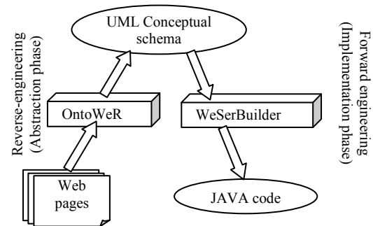
Figure 2. WA2WS framework.
