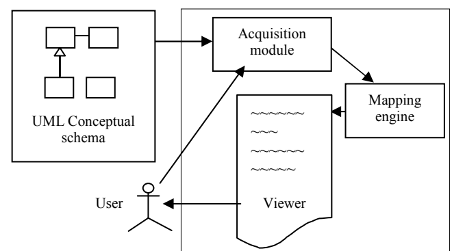
Figure 7. WeSerBuilder architecture.
