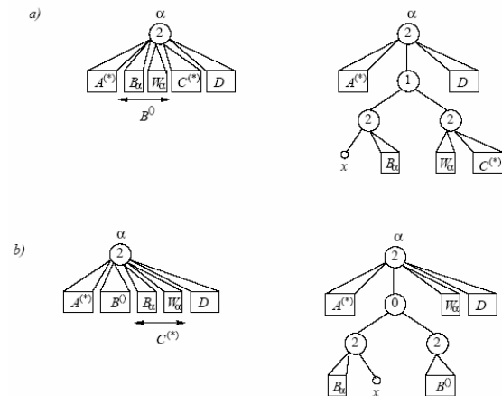
Figure 5. Construction of T' when \alpha has label 2, case 3.
