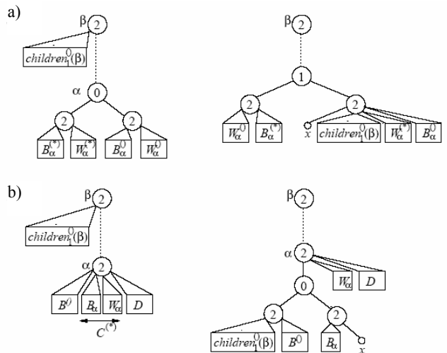
Figure 10. Construction of T' when \beta is a 2 misconfigured before \alpha and \gamma is not misconfigured.
