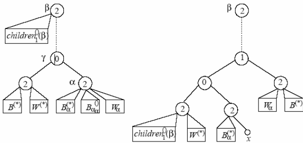
Figure 8. Construction of T' when \beta is a 2-misconfigured node before \alpha , \gamma is misconfigured and condition 1.b of theorem 8 holds.
