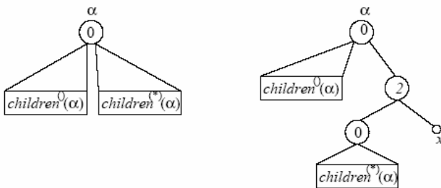
Figure 4. Construction of T' when \alpha has label 0, case 1.
