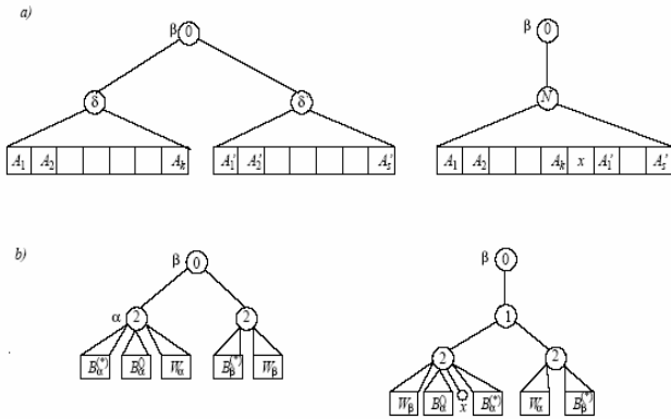
Figure 6. Construction of T' when \beta has label 0.
