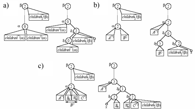
Figure 9. Construction of T' when \beta is a 2 misconfigured after \alpha and \gamma is not misconfigured.
