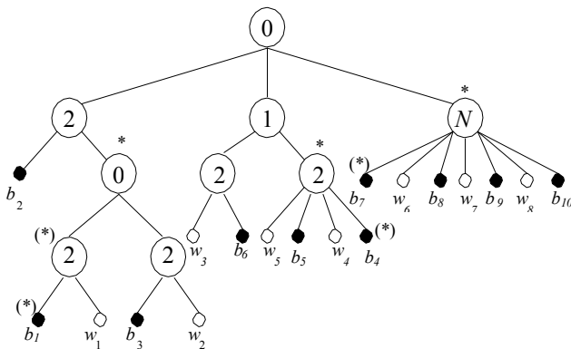
Figure 3. The marked tree for the illustrated graph in the Figure 2 when x is adjacent to b_1, b_4 and b_7 .
