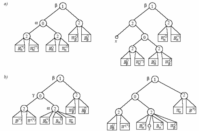
Figure 7. Construction of T when \beta has label 1, S = \{\alpha\} and condition c of Theorem 6 holds.
