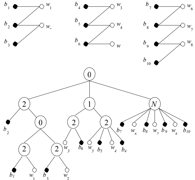
Figure 2. A bipartite graph Star_{123} -free and its extended canonical decomposition tree.
