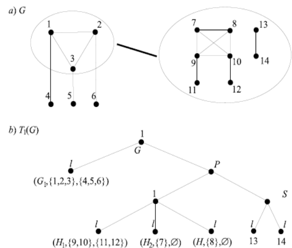
Figure 2. An example of a P_4 -sparse graph G and its tree T_1(G) .
