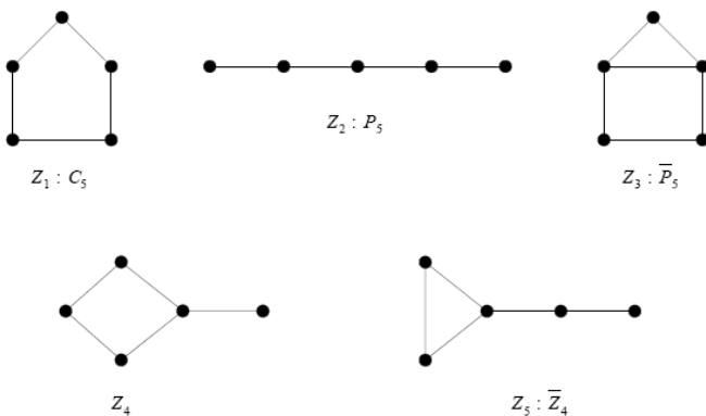
Figure 3. The set Z_{(1, P, S)} of graphs.
