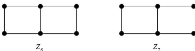
Figure 4. The graphs for Theorem 12.
