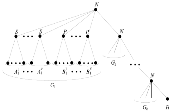
Figure 1. The modular decomposition tree of an 1-decomposable graph.
